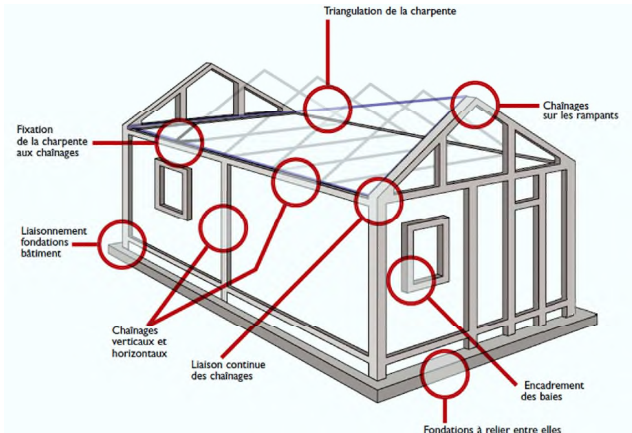
Structure monolithique Dispositions constructives (chaînages) © AGC / AFPS
