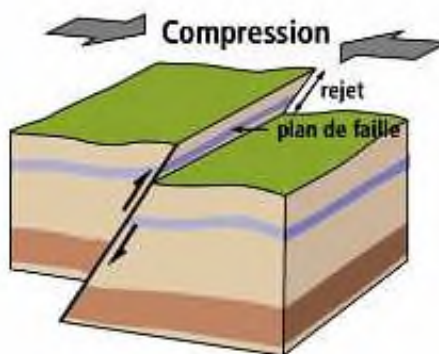
Faille inverse © BRGM
