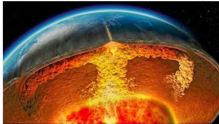
Cellule de convection
